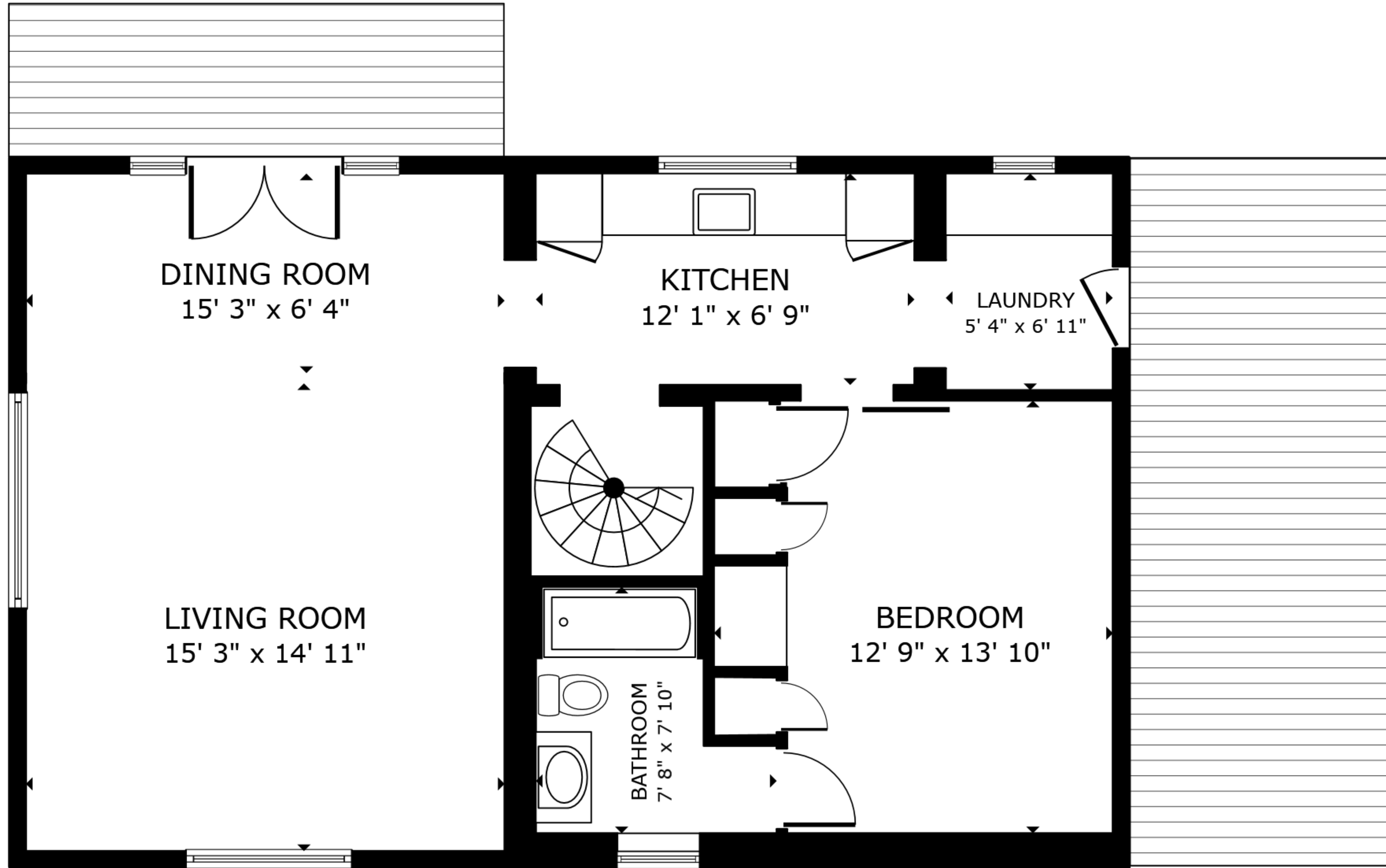
FLOOR 1
